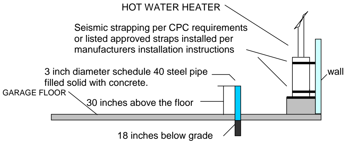
SECTION VIEW
