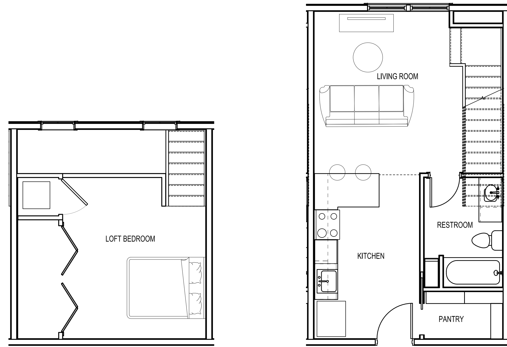
1 BLDG. "K" - TYPICAL LOFT UNIT 1/4"=1'-0"
