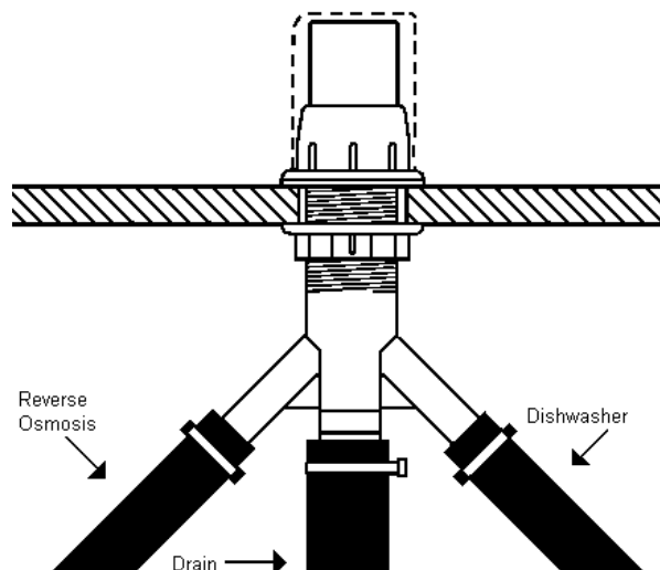
Reverse Osmosis with Dishwasher Example
