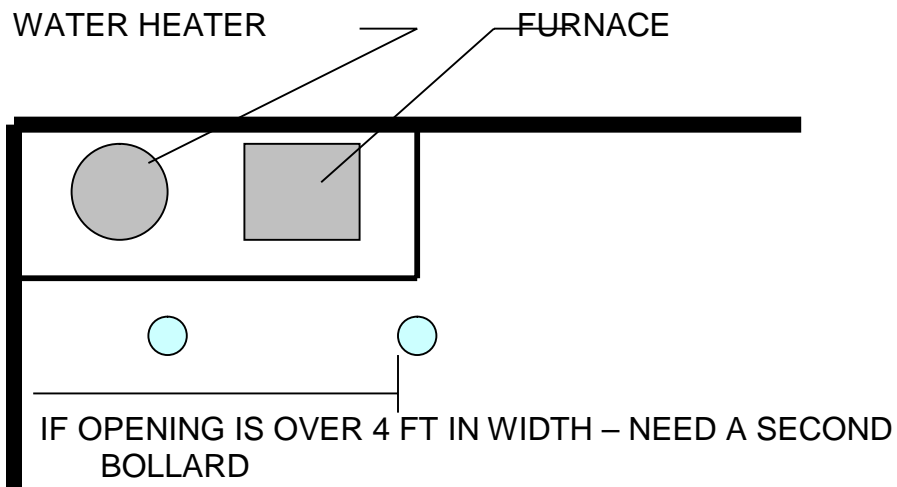
PLAN VIEW
