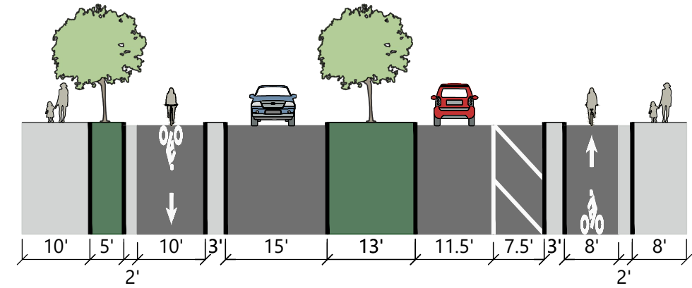
EXISTING CONDITIONS EL MACERO DR TO COWELL BLVD
