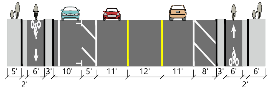
EXISTING CONDITIONS SAN MARINO DR TO EL MACERO DR
