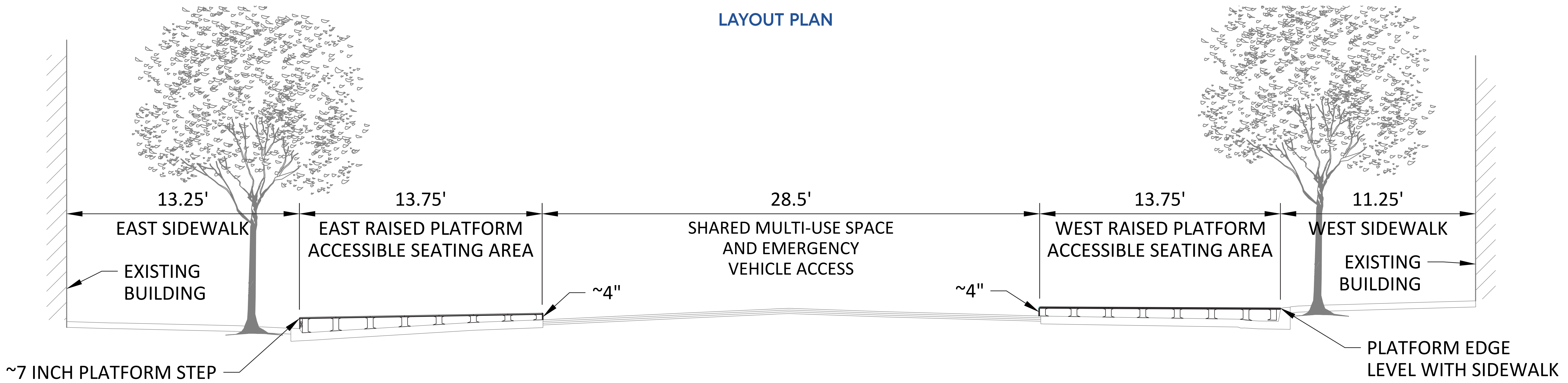
CROSS SECTION A-A
