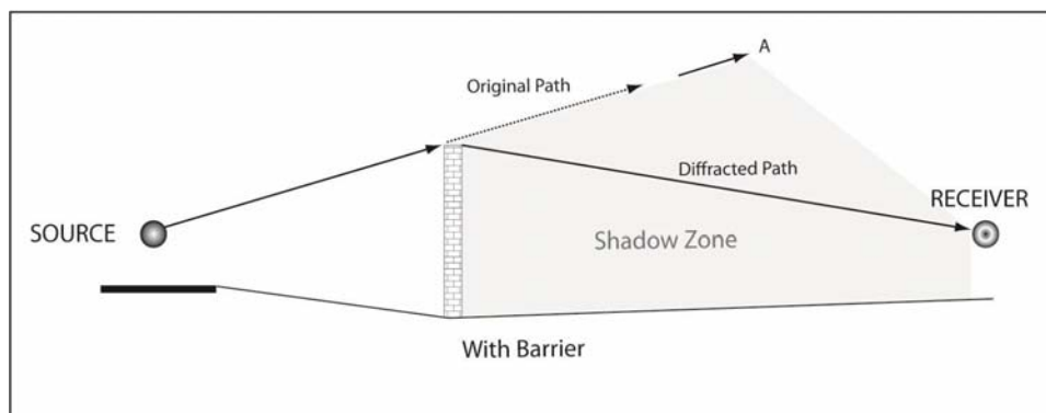
Figure 5-2. Barrier Diffraction
