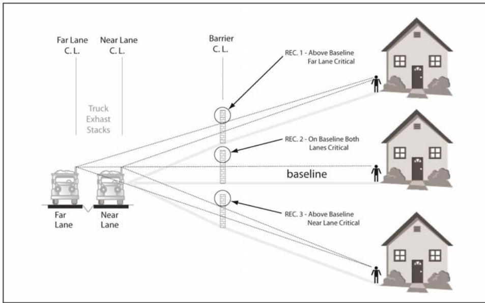
Figure 5-15. Determination of Critical Lane for Line-of-Sight Height
