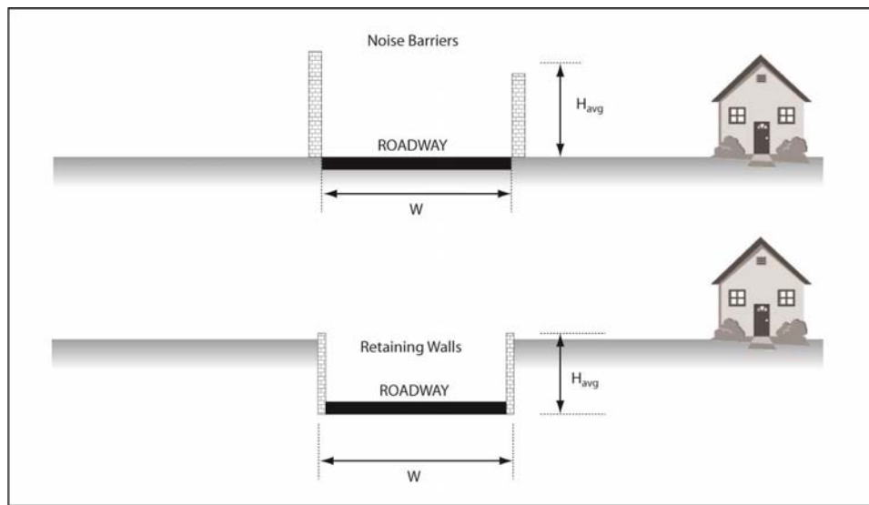
Figure 5-33. W / H_{AVG} Ratio Should be 10:1 or Greater
