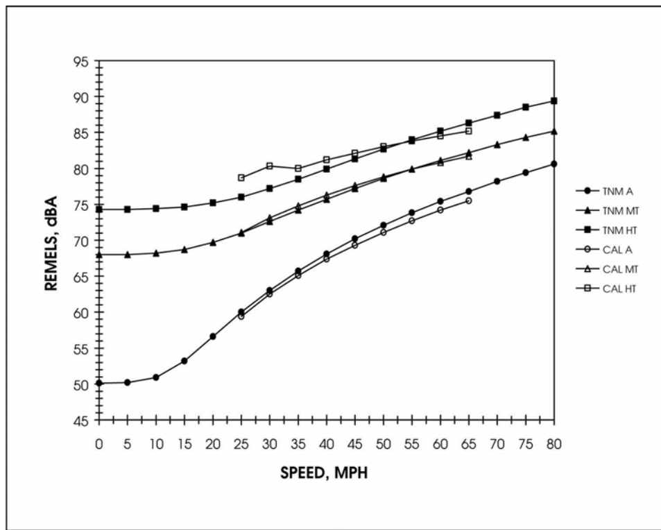
Figure 4-1. A-Weighted Baseline FHWA TNM REMEL Curves
