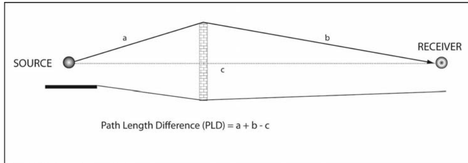
Figure 5-3. Path Length Difference
