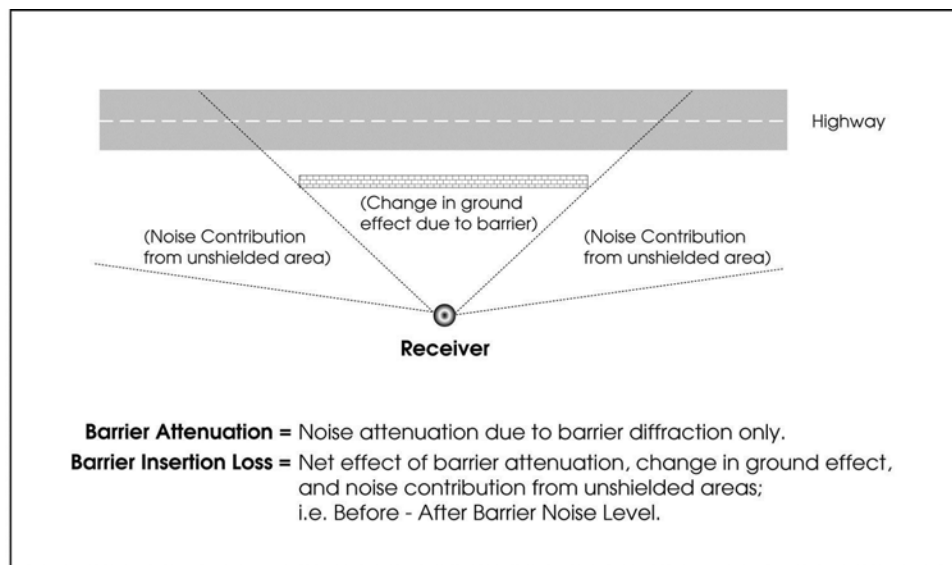
Figure 5-22. Barrier Insertion Loss vs. Attenuation
