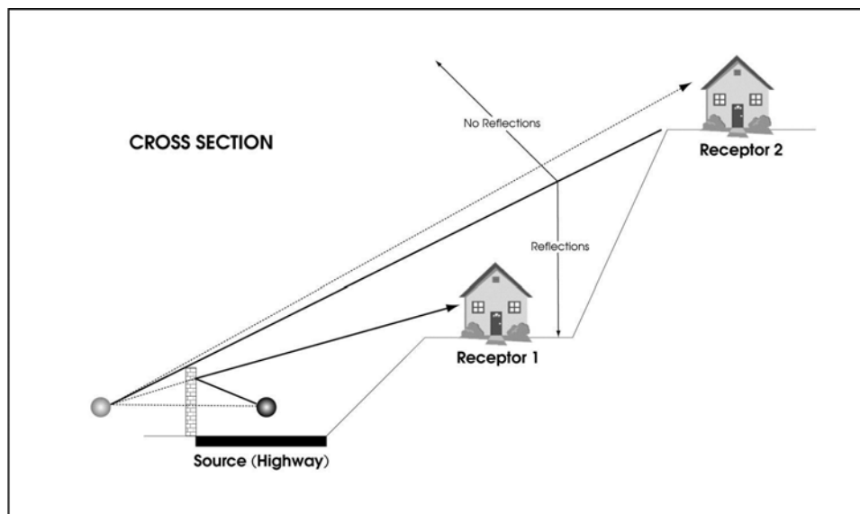
Figure 5-30. Placement of Image Sources (Cross Sectional View)
