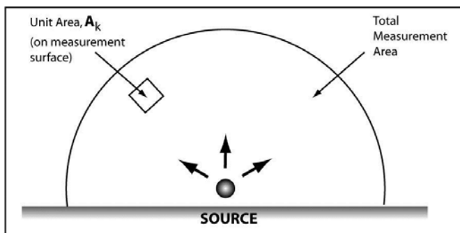
Figure 7-3. Sound Power Measurement Area
