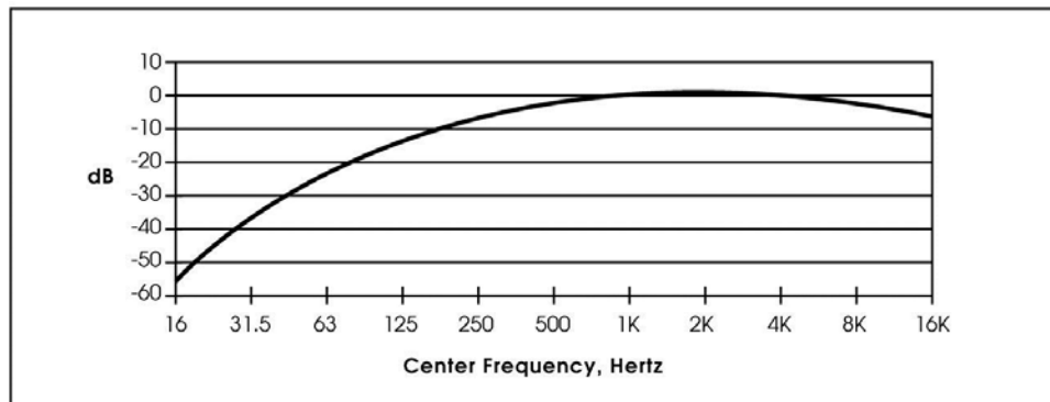
Figure 2-4. A-Weighting Network
