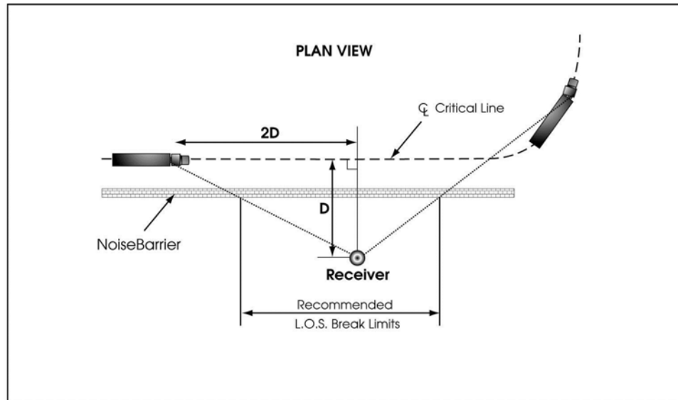
Figure 5-16. Recommended Line-of-Sight Break Limits
