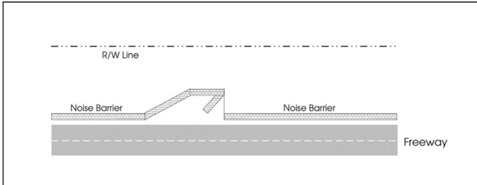
Figure 5-37. Barrier Offset with Solid Gate
