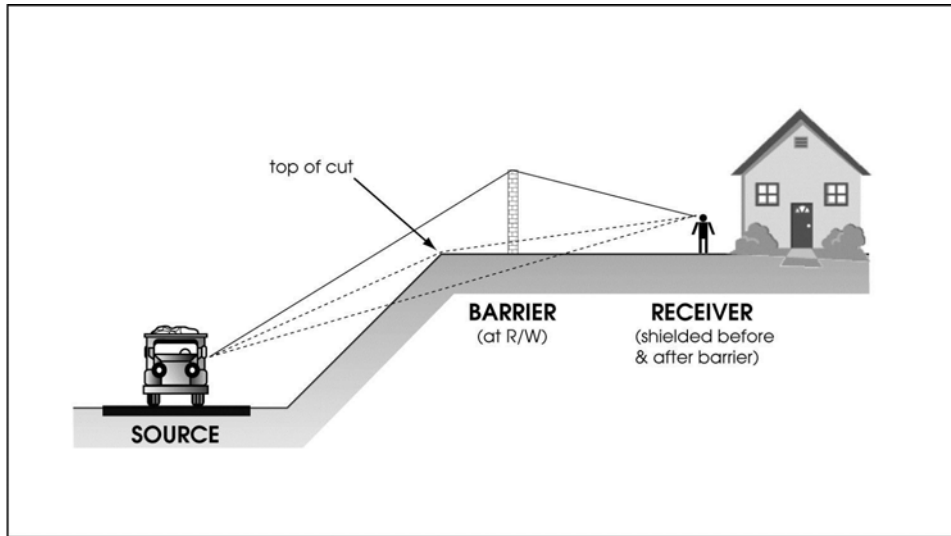
Figure 5-5. Typical Barrier Location for Depressed Highways
