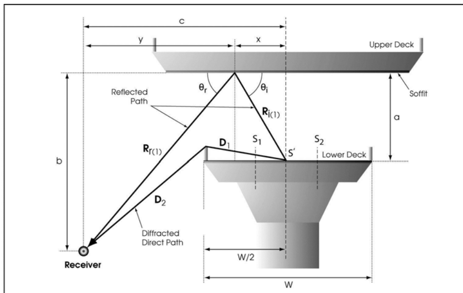
Figure 5-35. Double-Deck Structure Reflections, First Reflective Path
