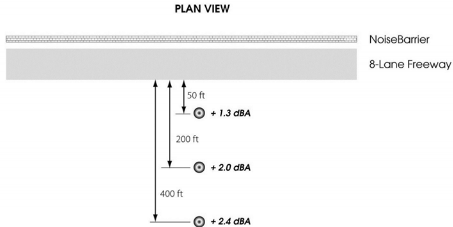
Figure 5-26. Noise Increases from Single-Barrier Reflections
