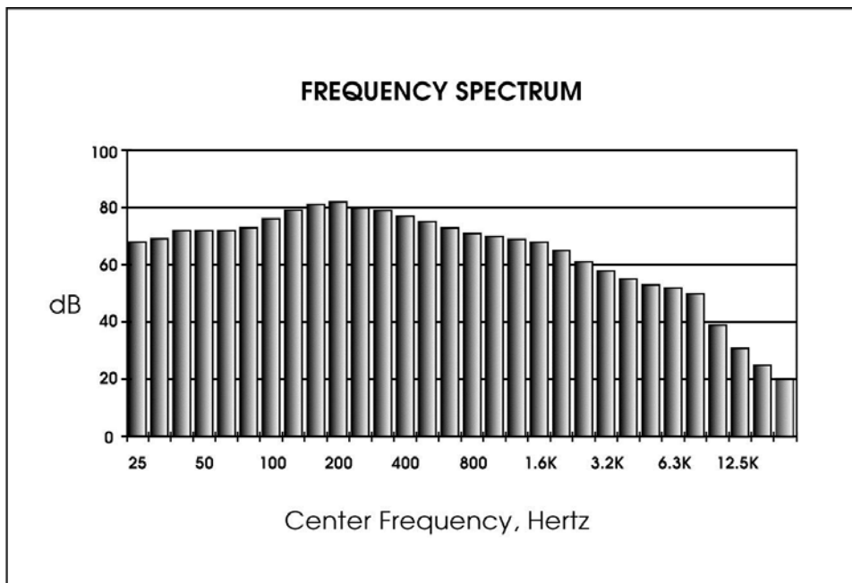
Figure 2-6. Typical One-Third-Octave Band Frequency Spectrum
