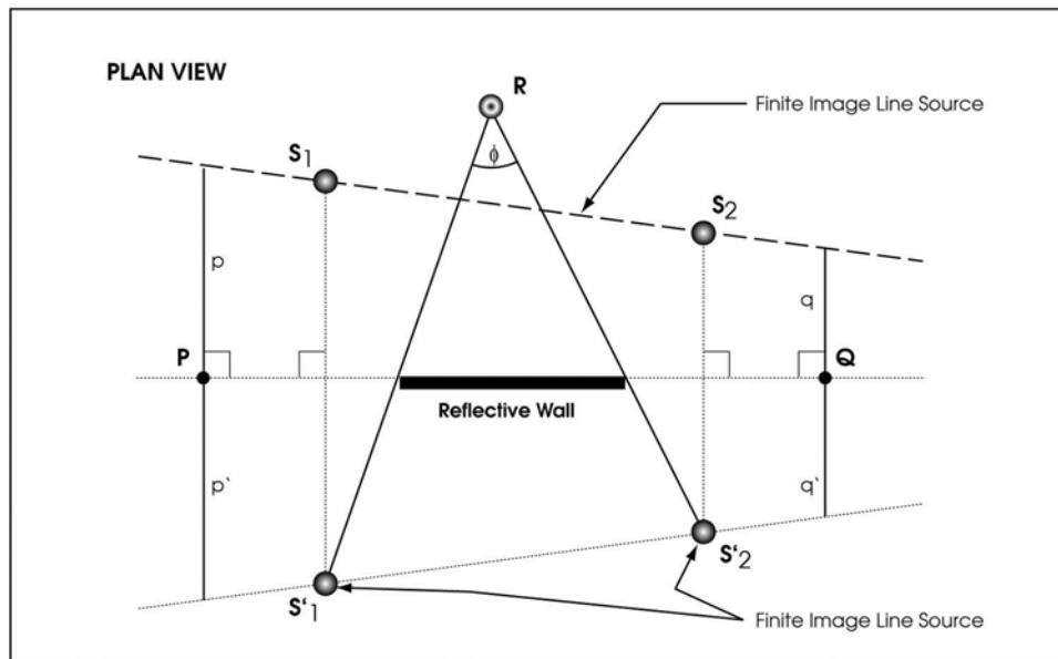
Figure 5-31. Placement of Image Sources (Plan View)
