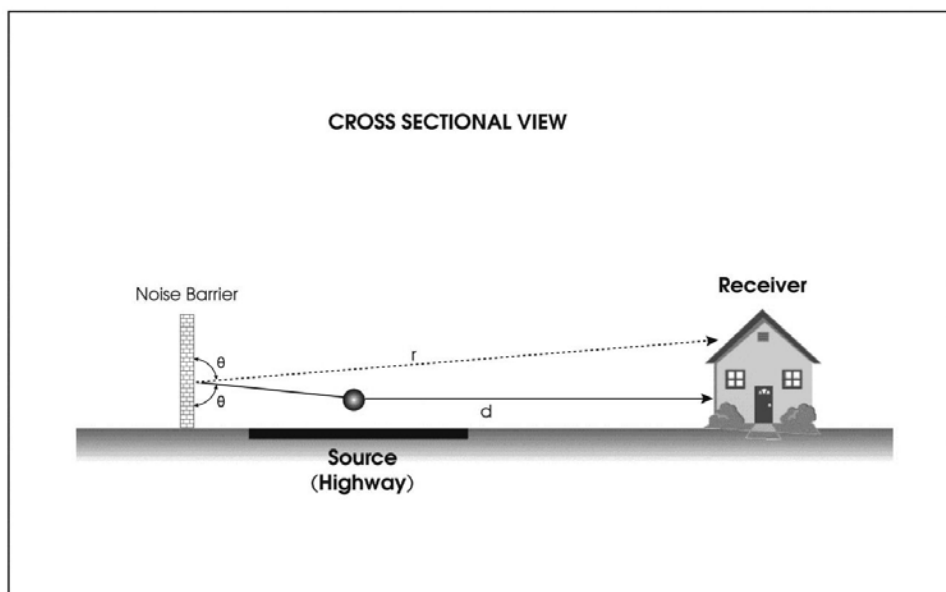
Figure 5-23. Single-Barrier Reflection (Simplest Representation)
