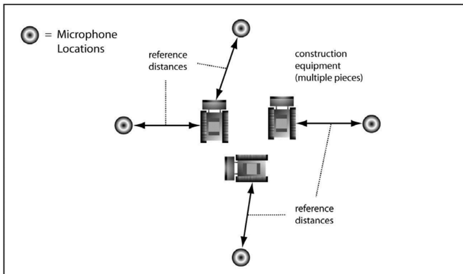
Figure 7-5. Measuring Multiple Pieces of Equipment Operating in Same Area
