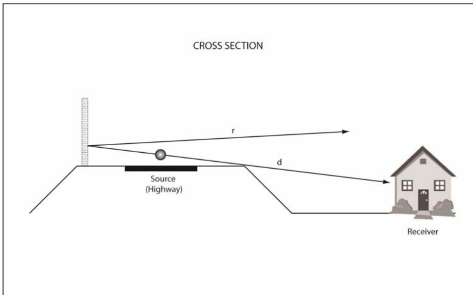
Figure 5-29. Highway and Noise Barrier on Fill
