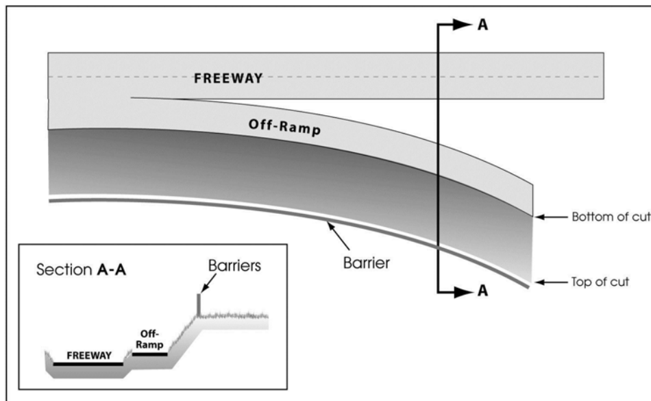
Figure 5-9. Barriers for Highway in Cut with Off-Ramp
