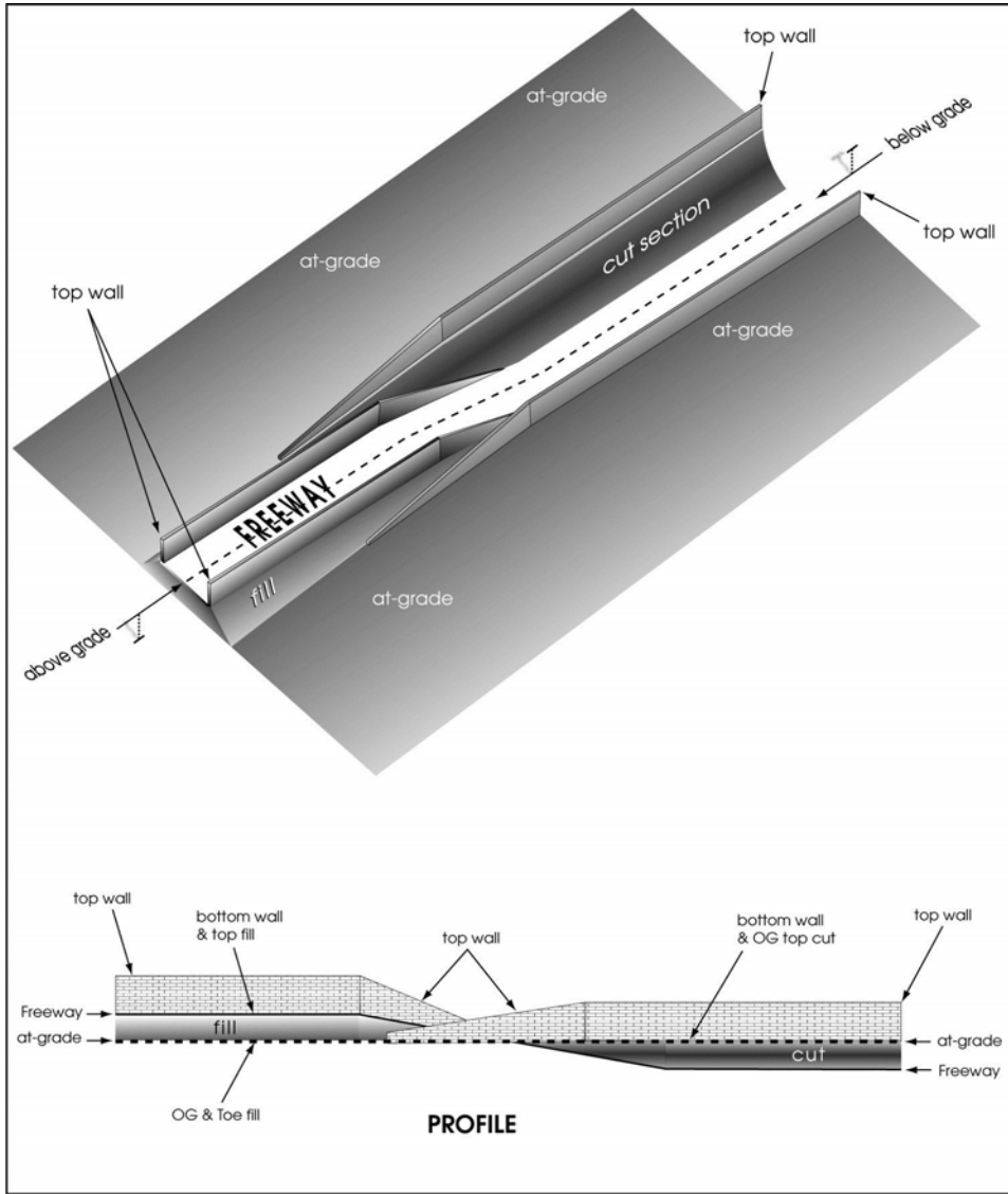
Figure 5-7. Barriers for Cut and Fill Transitions
