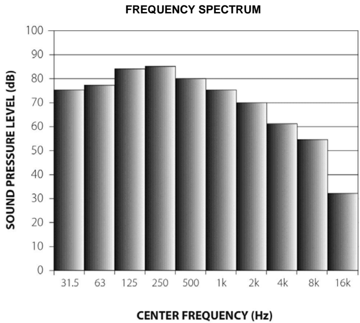
Figure 2-5. Typical Octave Band Frequency Spectrum
