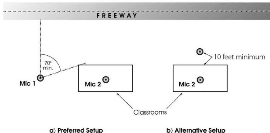
Figure 3-4. Classroom Noise Measurements (Reconstruction of Existing Freeway)
