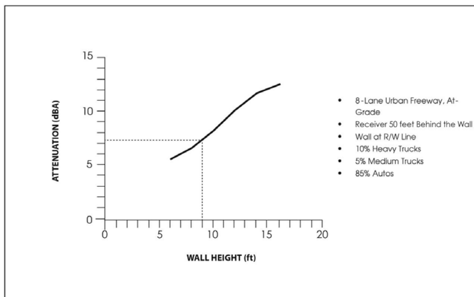
Figure 5-12. Soundwall Attenuation vs. Height for At-Grade Freeway
