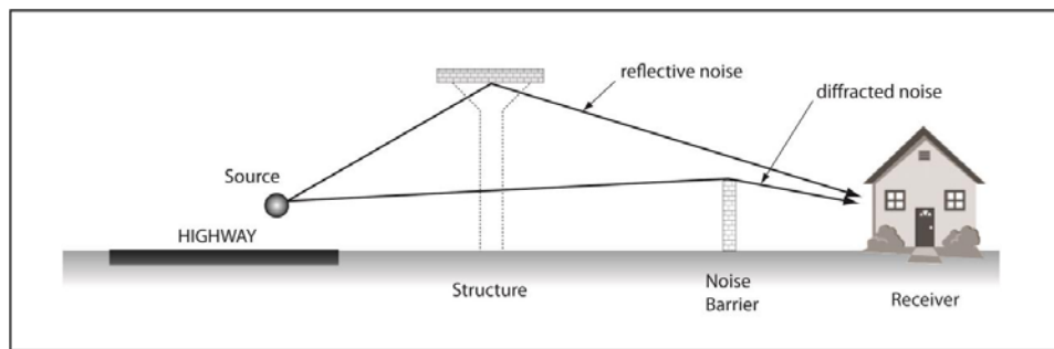
Figure 5-34. Noise Reflection off Structure
