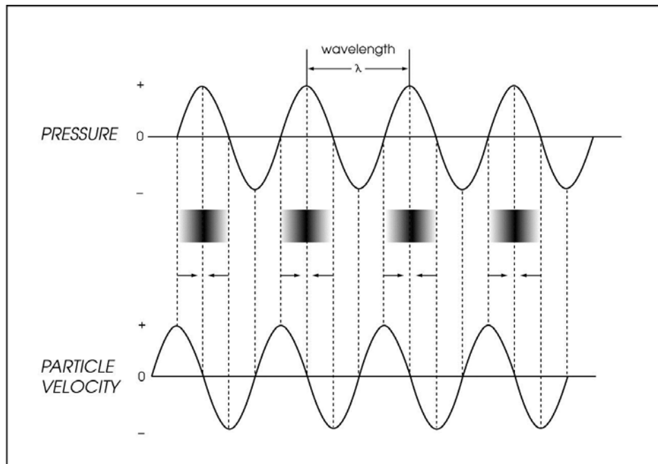
Figure 2-1. Sound Pressure vs. Particle Velocity
