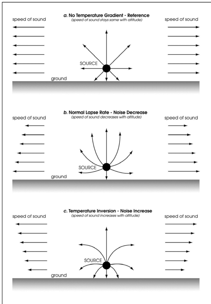
Figure 2-11. Effects of Temperature Gradients on Noise
