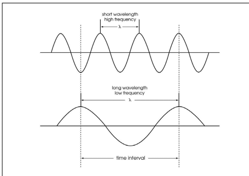
Figure 2-2. Frequency and Wavelength
