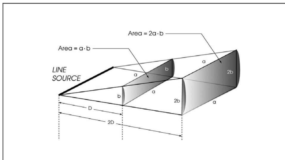
Figure 2-9. Line Source Propagation (Cylindrical Spreading)
