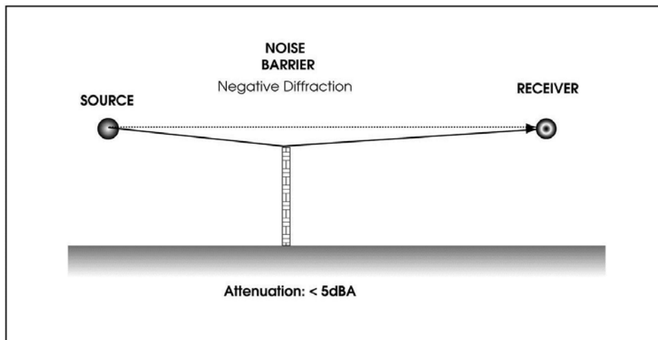
Figure 2-17. Negative Diffraction, Which Provides Some Noise Attenuation
