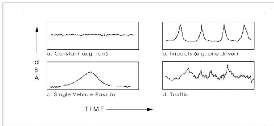
Figure 2-18. Different Noise Level vs. Time Patterns
