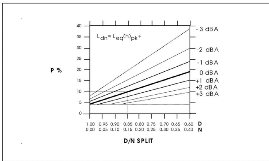
Figure 2-19. Relationship between L_{dn} and L_{eq}(h)_{pk}
