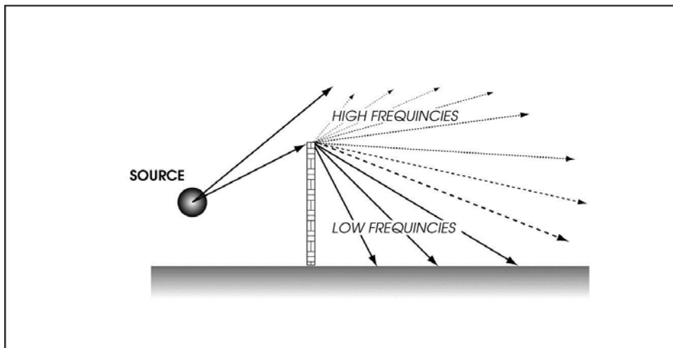
Figure 2-13. Diffraction of Sound Waves
