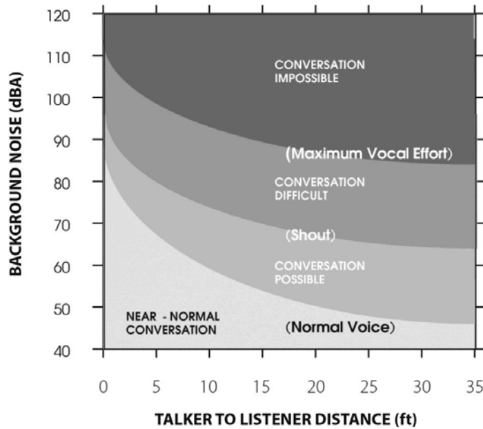
Figure 2-20. Interference of Conversation from Background Noise
