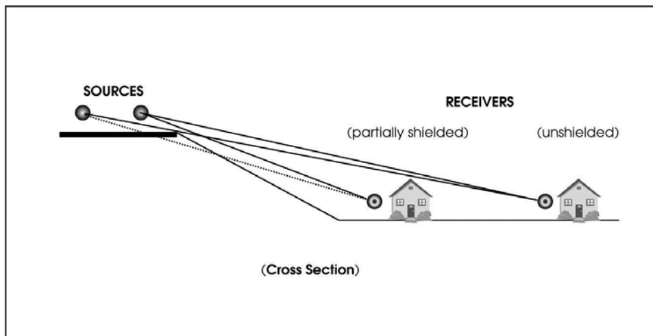
Figure 3-2. Typical Noise Measurement Site Locations
