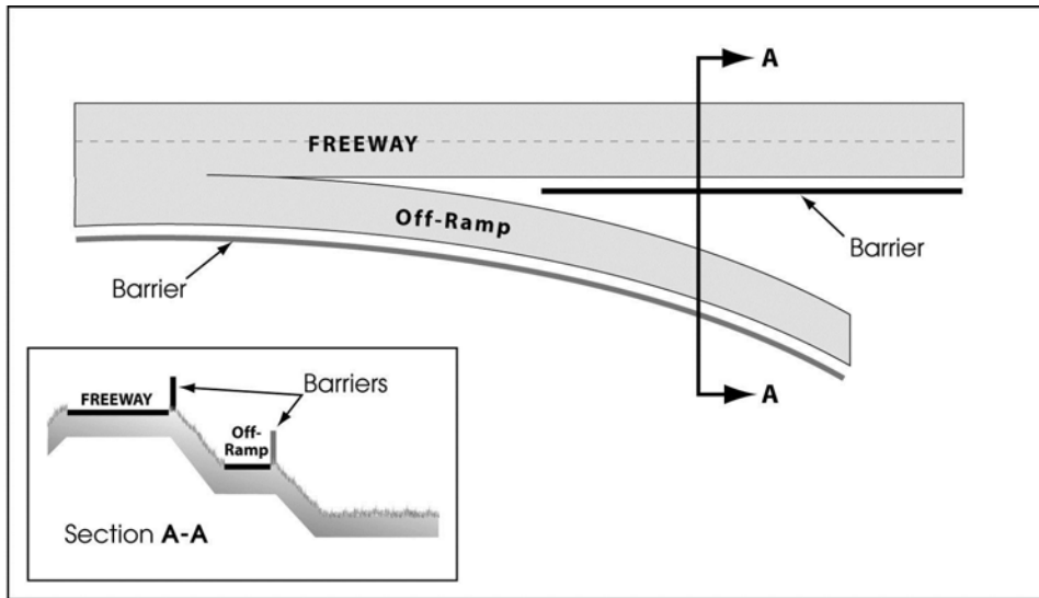
Figure 5-8. Barriers for Highway on Fill with Off-Ramp
