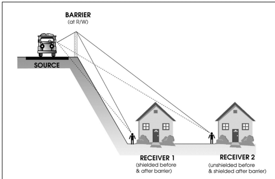
Figure 5-6. Typical Barrier Location for Elevated Highways
