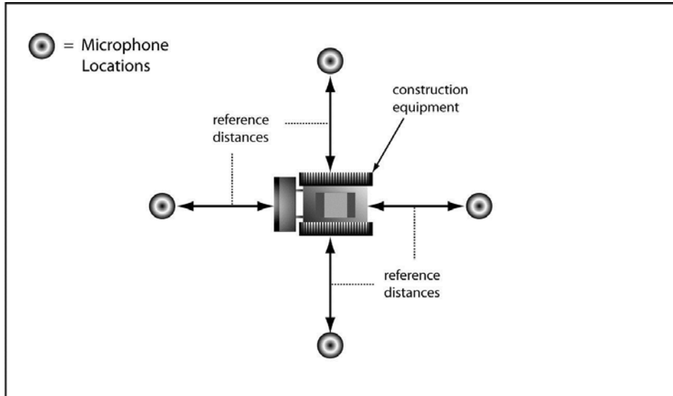
Figure 7-4. Measuring One Piece of Equipment
