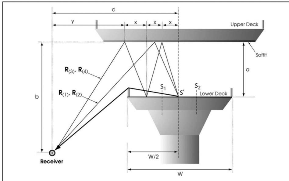
Figure 5-36. Multiple Reflective Paths
