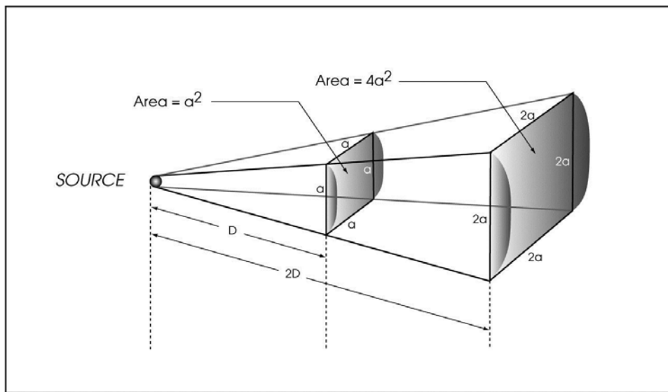
Figure 2-7. Point Source Propagation (Spherical Spreading)
