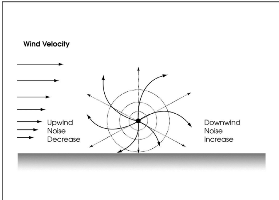
Figure 2-10. Wind Effects on Noise Levels
