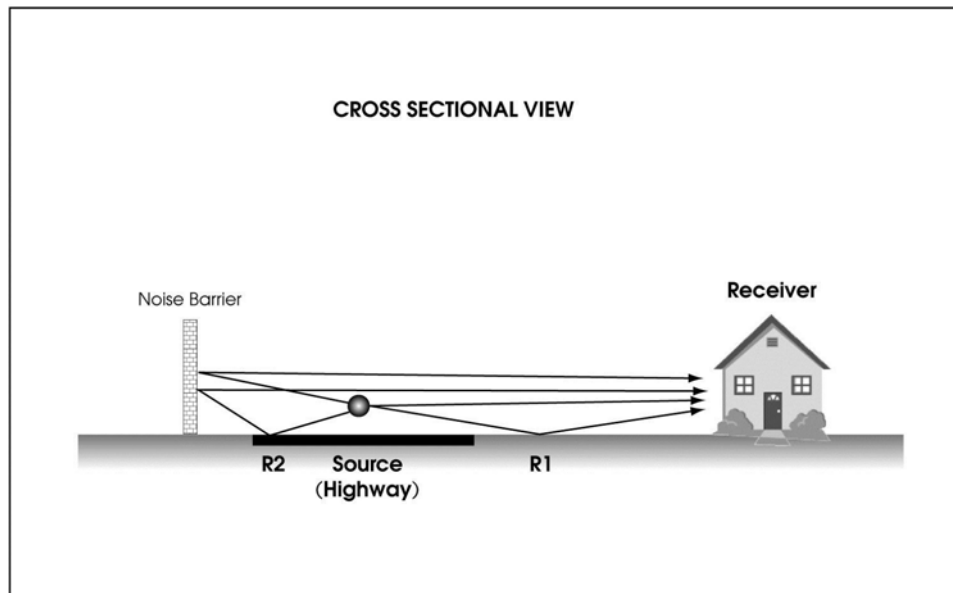
Figure 5-25. Single-Barrier Reflection (More Accurate Representation)
