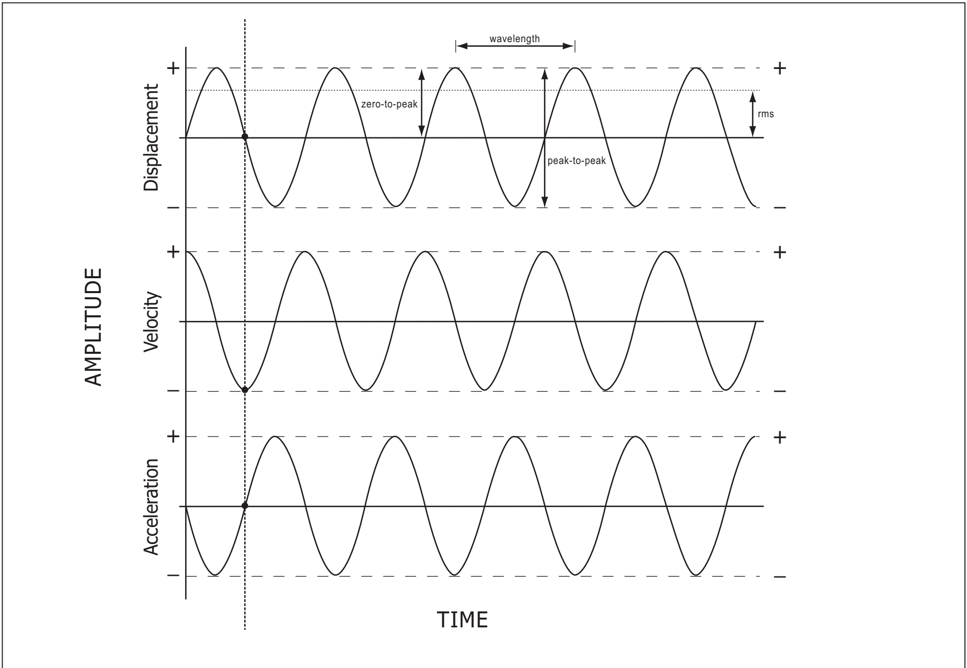
Figure 2 Quantities Used to Describe Vibratory Motion
