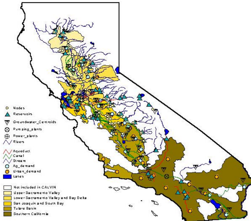
Figure 1. Demand Areas and Major Inflows and Facilities Represented in CALVIN
