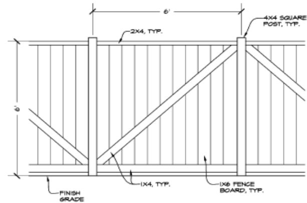
2 6' HIGH SOLID FENCE SECTION 1/2" = 1'-0"
