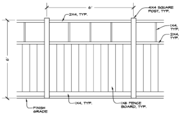
1 6' HIGH PARTIALLY OPEN FENCE SECTION 1/2" = 1'-0"
