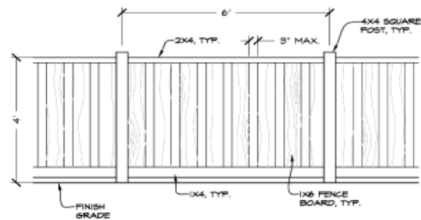
4 4' HIGH OPEN FENCE AT COMMUNITY GARDEN SECTION 1/2" = 1'-0"
