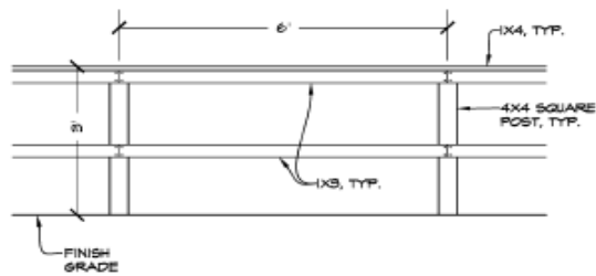
3 3' HIGH FARM FENCE SECTION 1/2" = 1'-0"
